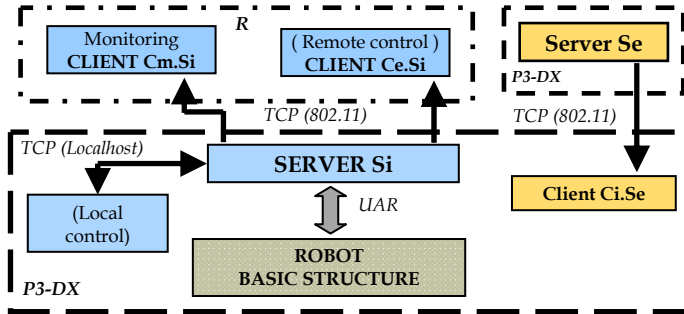
Fig. 7. Proposal of client-server architecture based on Player/Stage for the development of telerobotics application with P3-DX units.
