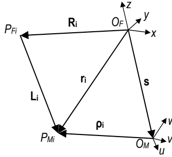
Fig. 4. Single kinematic chain of a parallel device.
