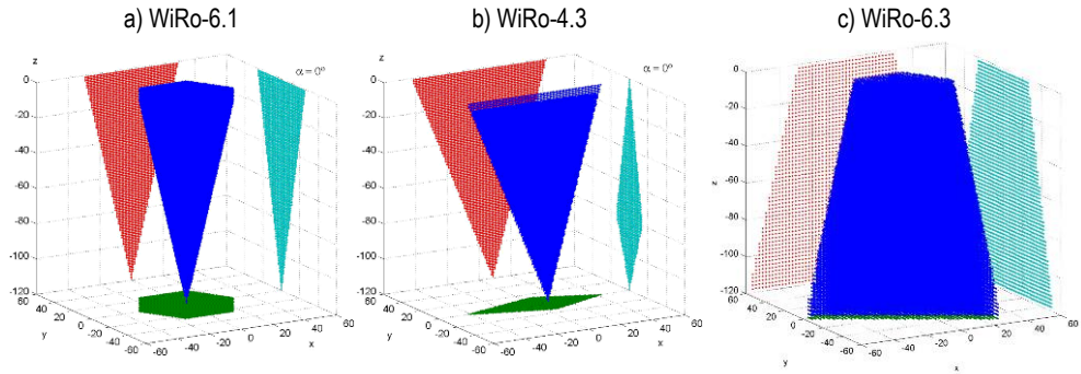
Fig. 5. Positional workspace of the three structures considered.
