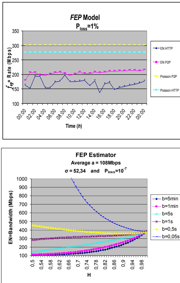
Fig. 10. Bandwidth estimation curves using the FEP method.
