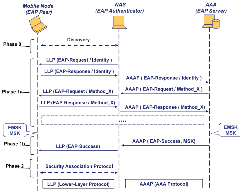
Fig. 3. EAP authentication exchange
