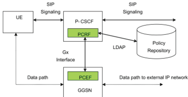
Fig. 10. Policy architecture in UMTS IMS
