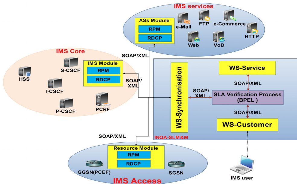
Fig. 11. SLM&M distributed architecture.
