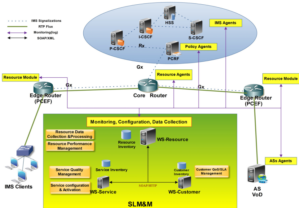
Fig. 13. Centralized trial infrastructure.
