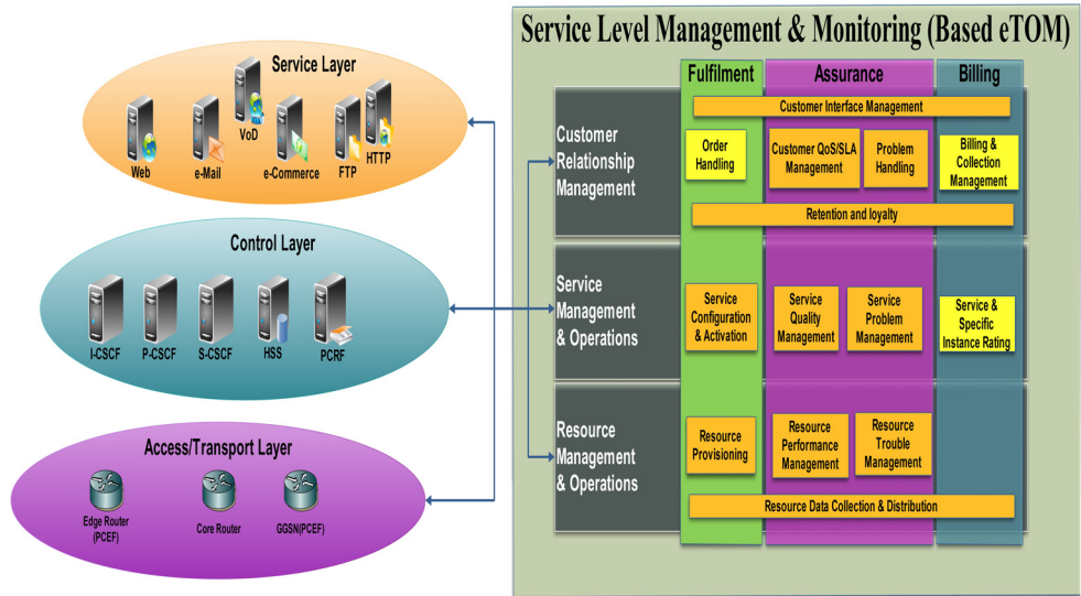
Fig. 8. eTOM and IMS interactions.
