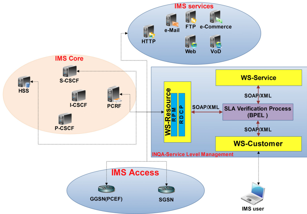
Fig. 10. SLM&M Centralized architecture.
