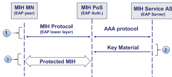
Fig. 8. MIH protocol as EAP lower-layer
