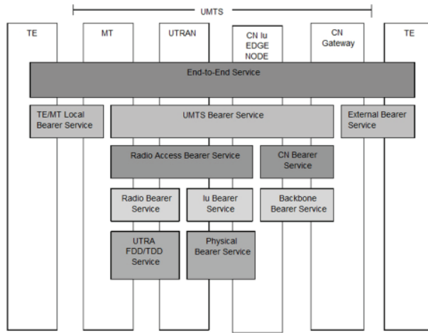
Fig. 1. UMTS QoS architecture
