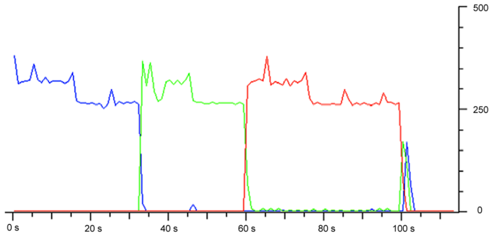
Fig. 9. TCP concurrent flows with QoS (bit/s).
