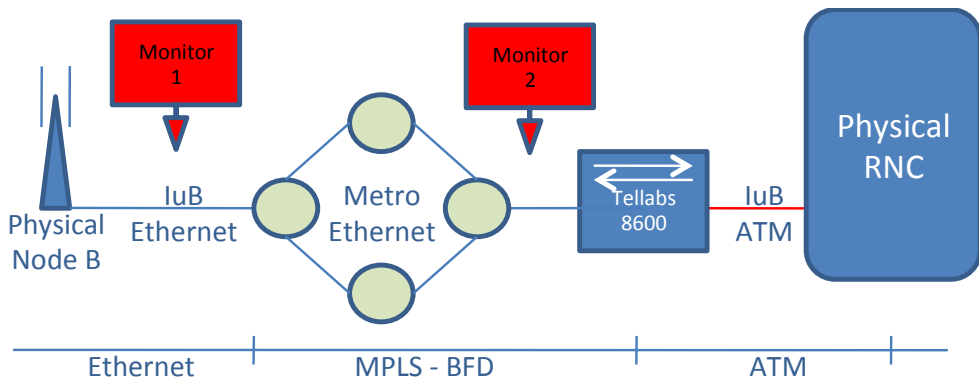
Fig. 11. 3G Network.
