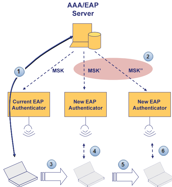
Fig. 11. Key pre-distribution mechanism
