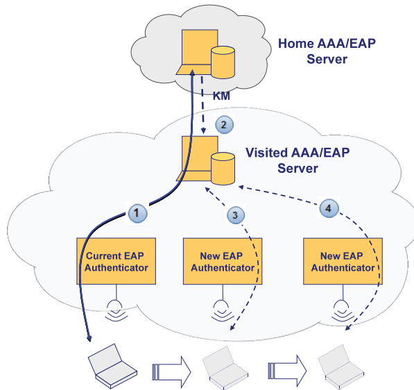
Fig. 12. Use of a local server mechanism
