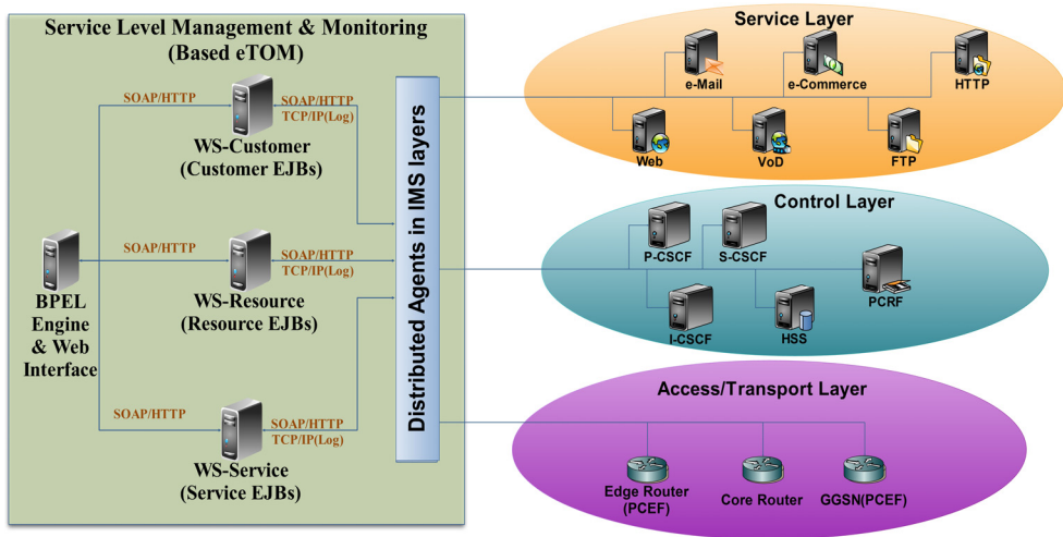
Fig. 9. Implementation architecture.
