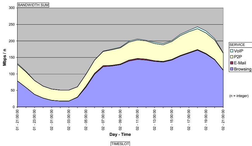
Fig. 5. Downstream traffic “on peak” and “off peak”. Traffic rate is normalized, 24 hours sampled (De Deus, 2007).
