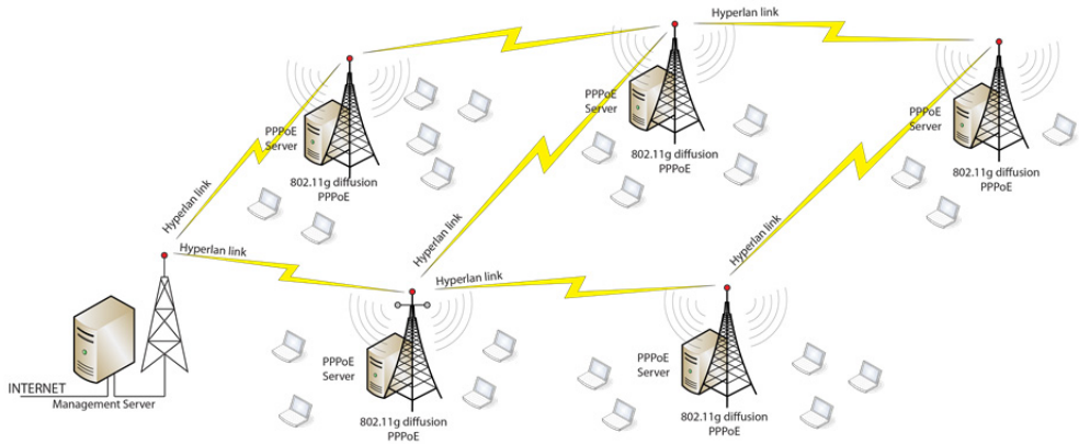
Fig. 14. first extended testbed scenario.
