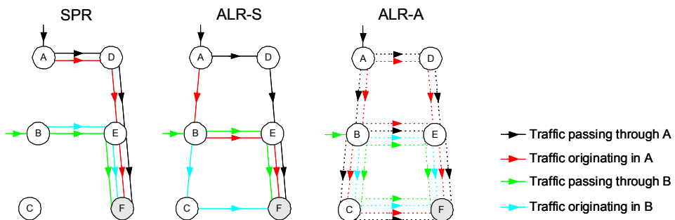
Fig. 1. Path selection with different forwarding policies.
