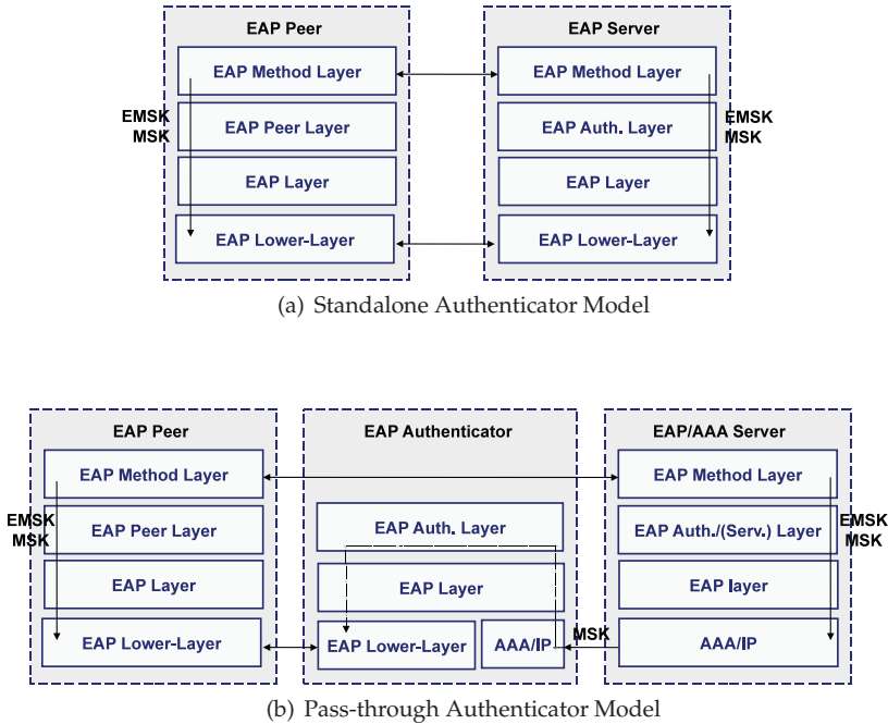
Fig. 2. EAP authenticator models
