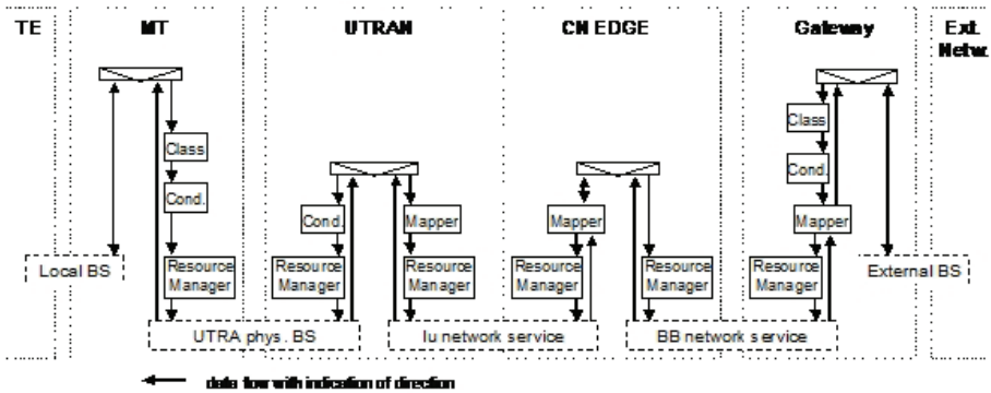
Fig. 4. QoS management function for UMTS bearer service in the user plane
