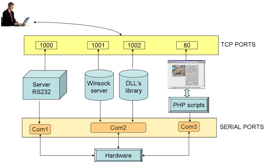
Fig. 4. Communication tier.
