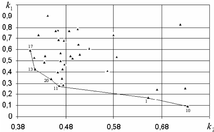
Fig. 1. Choice of Pareto-optimal variants of the telecommunication network.
