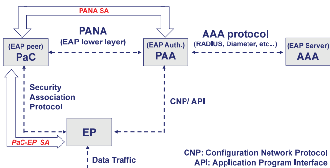
Fig. 7. PANA architecture
