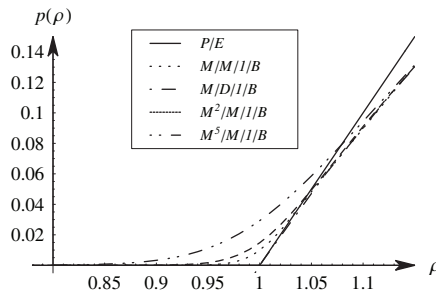
Fig. 6. Comparison of different queueing models.
