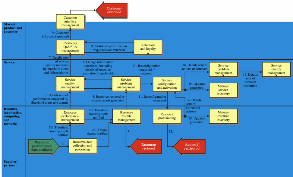
Fig. 7. Processes Flow in SLA execution with violation.
