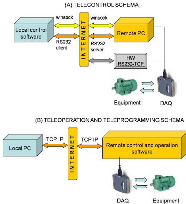
Fig. 2. Telecontrol, teleoperation and teleprogramming schema.
