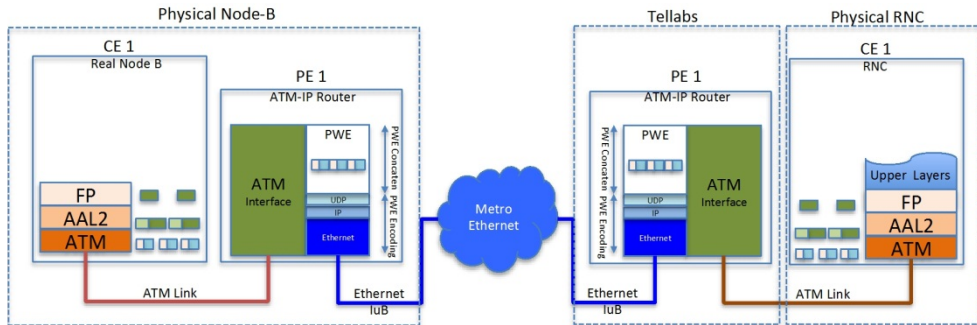
Fig. 12. 3G topology from Node B to RNC.
