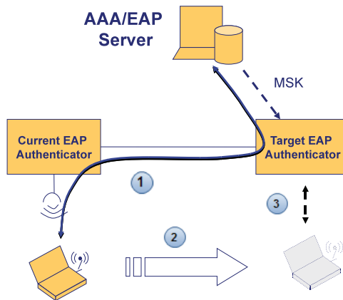
Fig. 10. Pre-authentication mechanism
