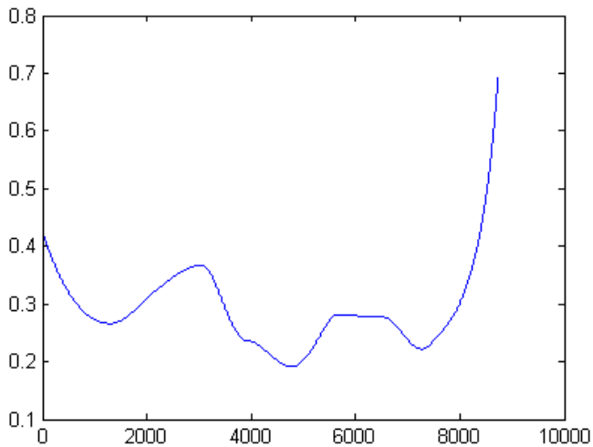
Fig. 16. 3G Traffic multifractal analysis – Hölder function. (milliseconds time scale).
