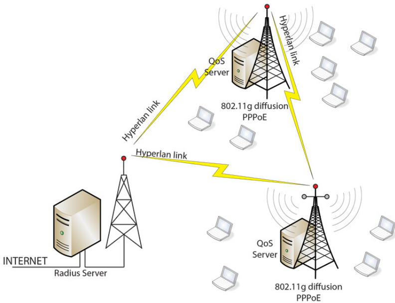
Fig. 15. second extended testbed scenario.
