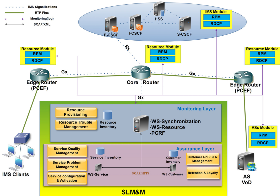
Fig. 14. Centralized trial infrastructure.
