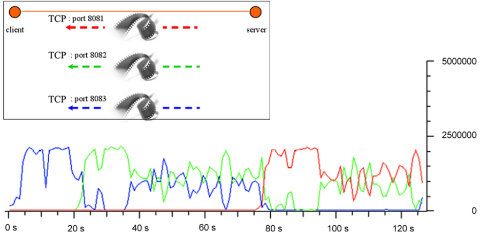
Fig. 8. three concurrent videos with QoS (bit/s).
