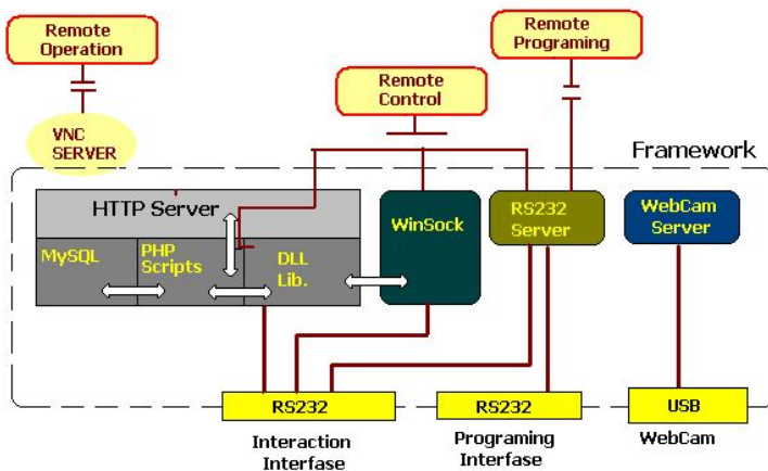
Fig. 3. Multitier architecture proposed.
