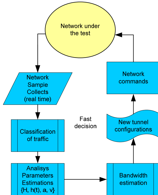
Fig. 8. Proposal of a network real-time forecast framework with bandwidth estimation.
