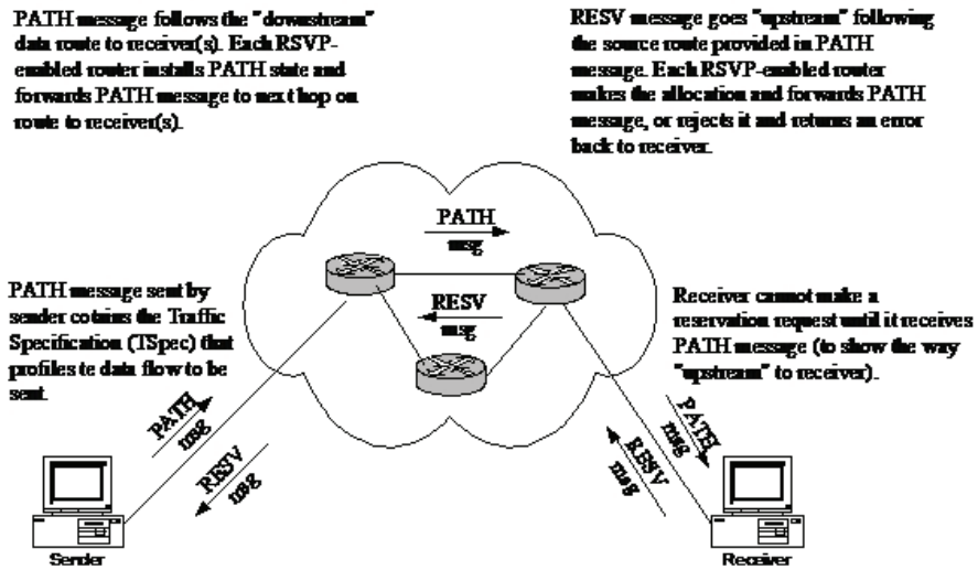
Fig. 5. RSVP setup flow
