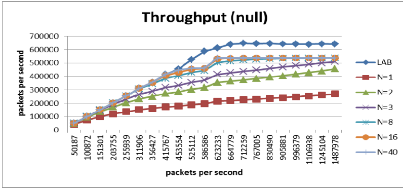
Fig. 18. Theoretical and experimental throughputs without analysis load.
